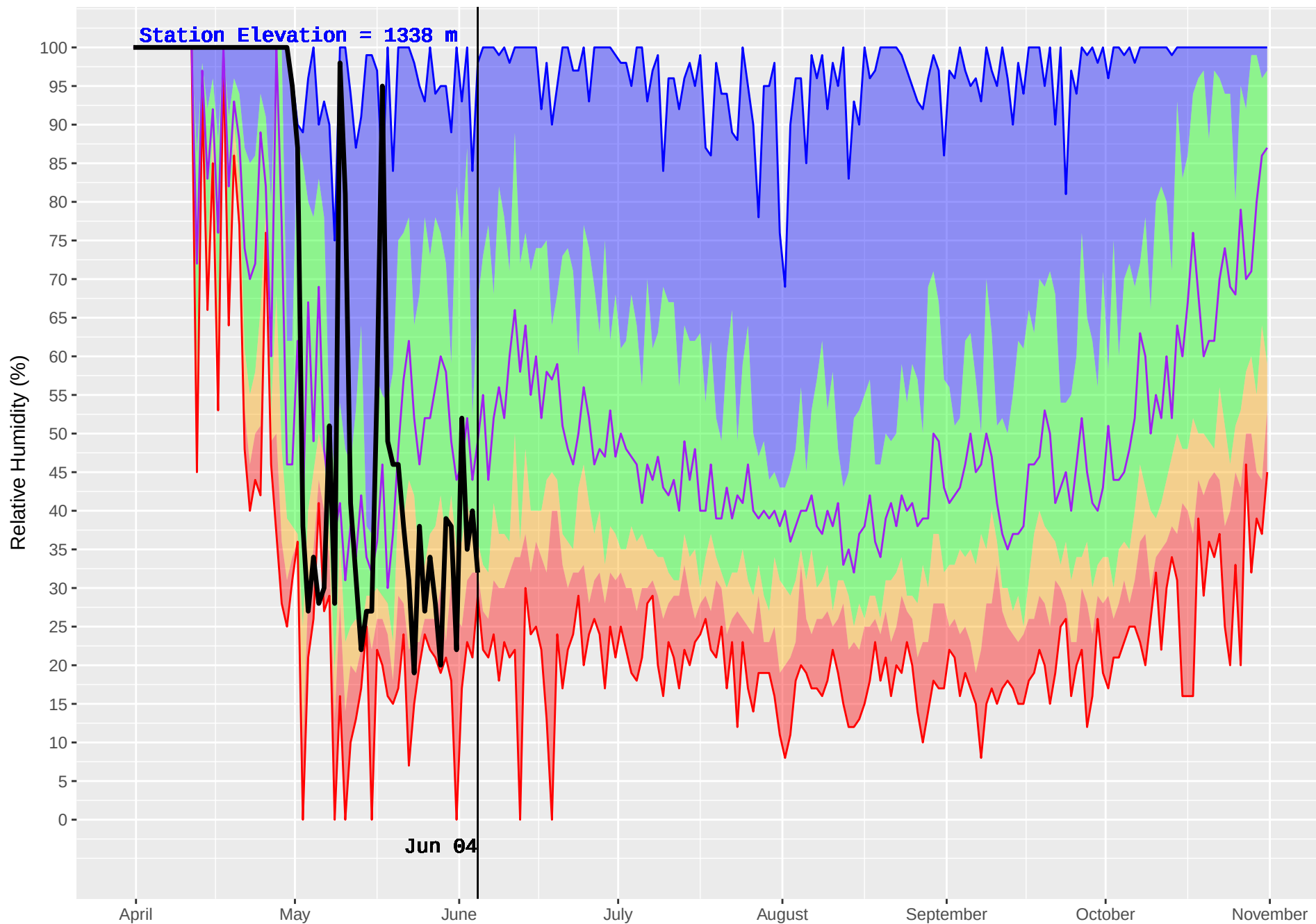
EIGHT MILE (391) : Historical (1980–2016) and Current (2018) Noon Relative Humidity
