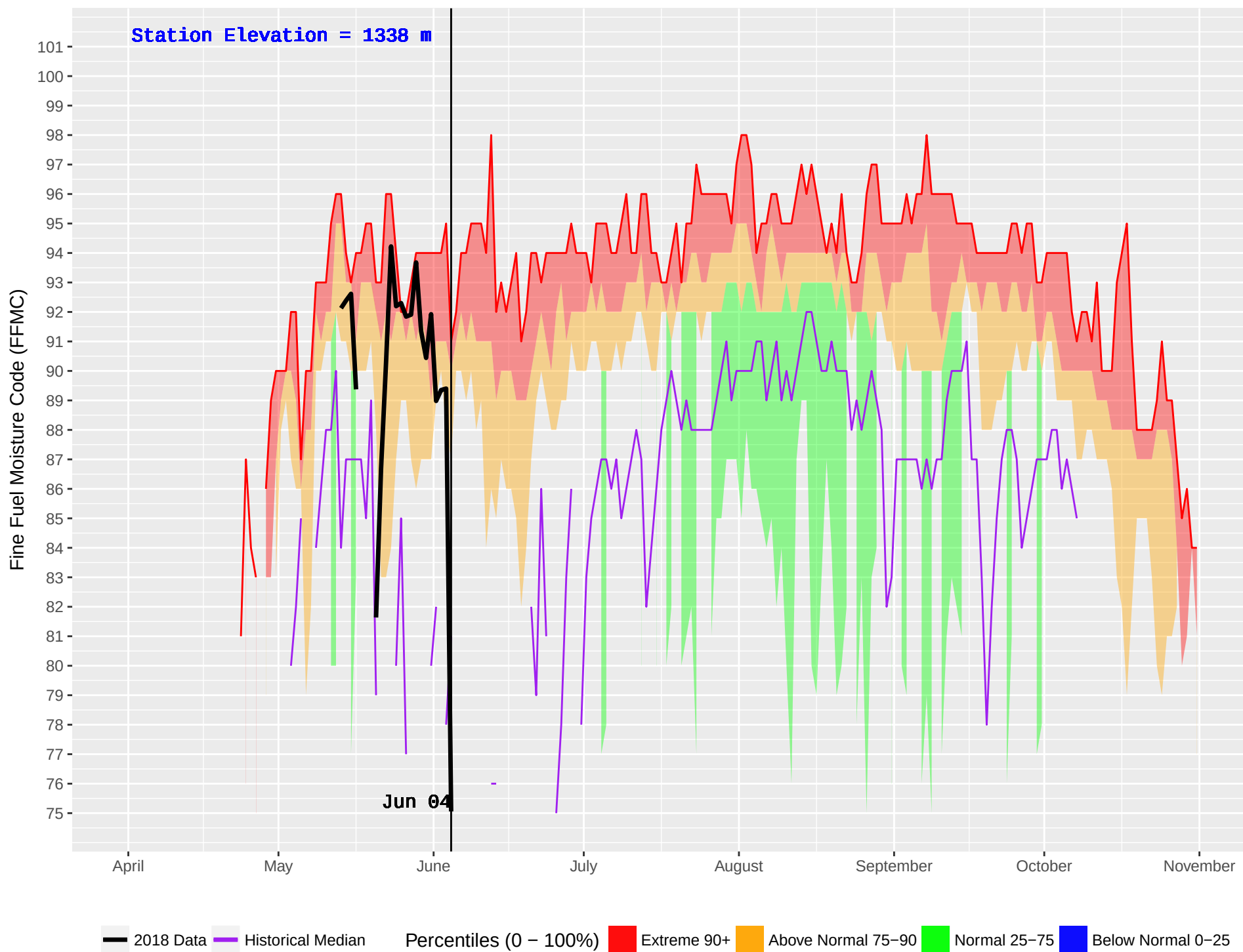
EIGHT MILE (391) : Historical (1980–2016) and Current (2018) Noon Fine Fuel Moisture Code (FFMC)
