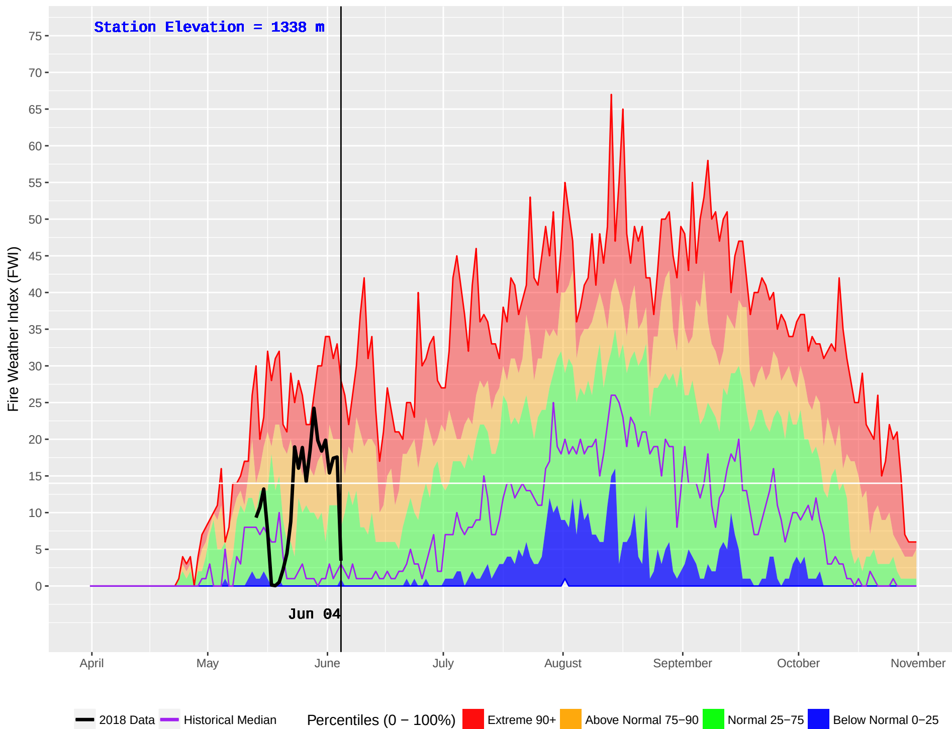
EIGHT MILE (391) : Historical (1980–2016) and Current (2018) Noon Fire Weather Index (FWI)
