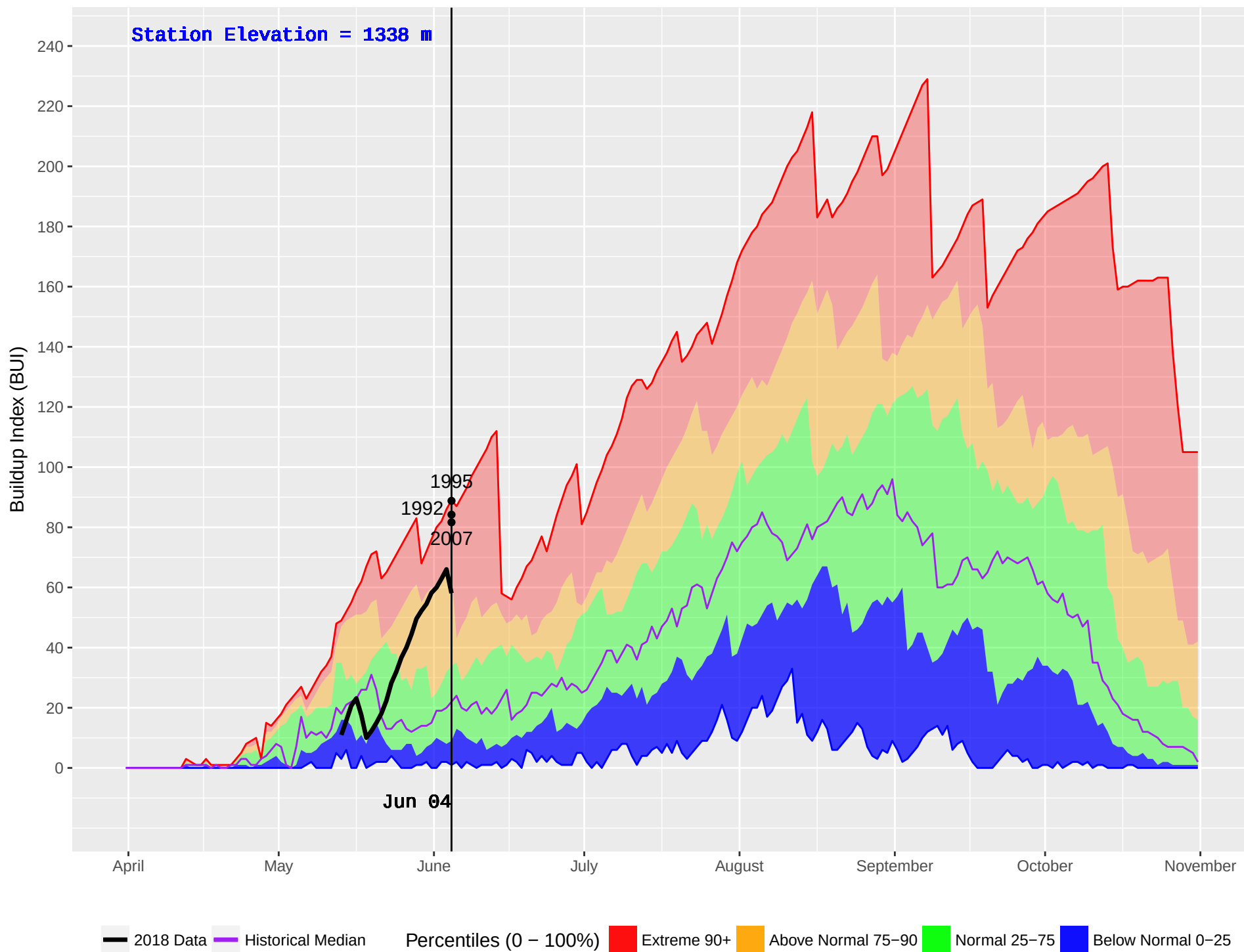
EIGHT MILE (391) : Historical (1980–2016) and Current (2018) Noon Buildup Index (BUI)
